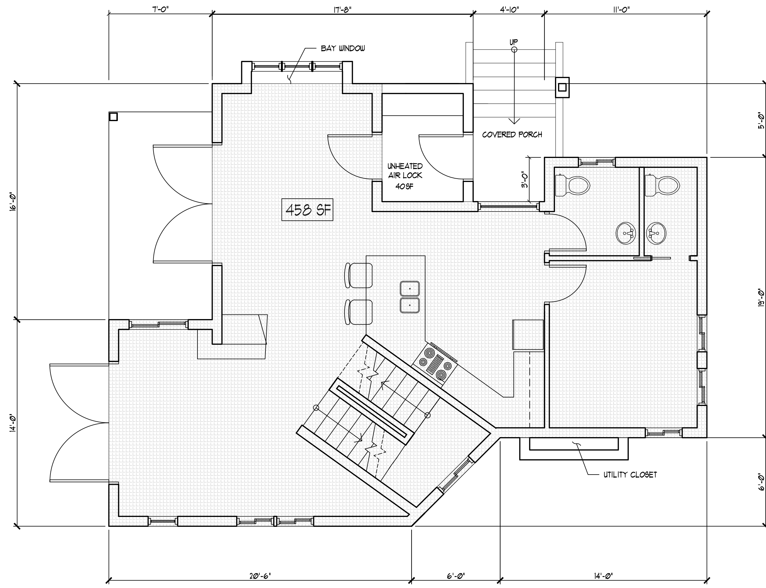
1 First Floor 03 SCALE: 1/4"=1' 458 SF (HEATED) 40 SF (UNHEATED)
