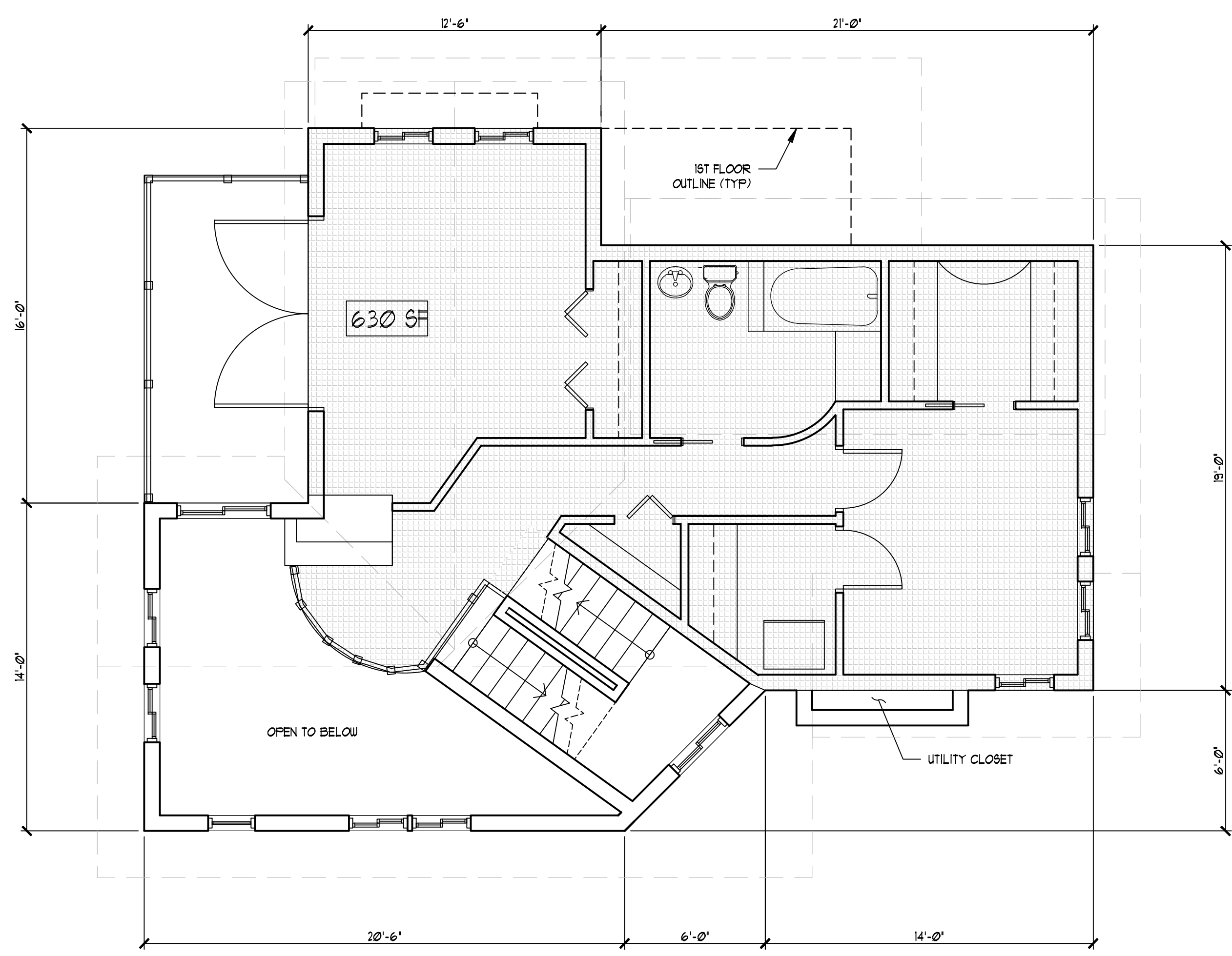
2 Second Floor 03 SCALE: 1/4"=1' 630 SF (HEATED)
