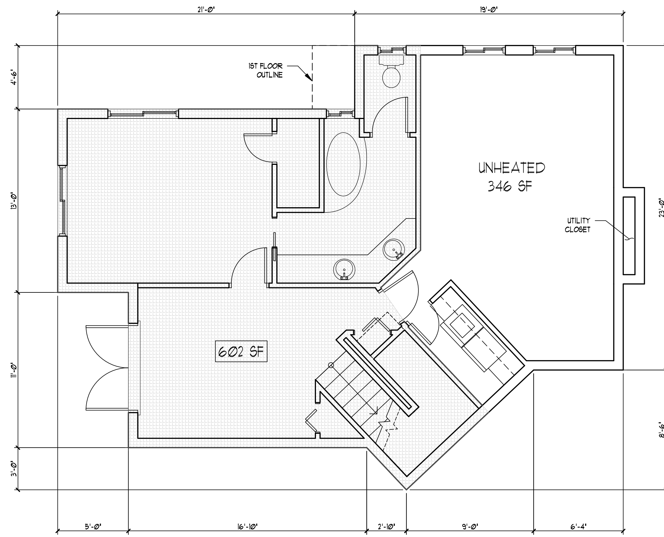
1 Basement 06 SCALE: 1/4"=1' 602 SF (HEATED) 346 SF (UNHEATED)
