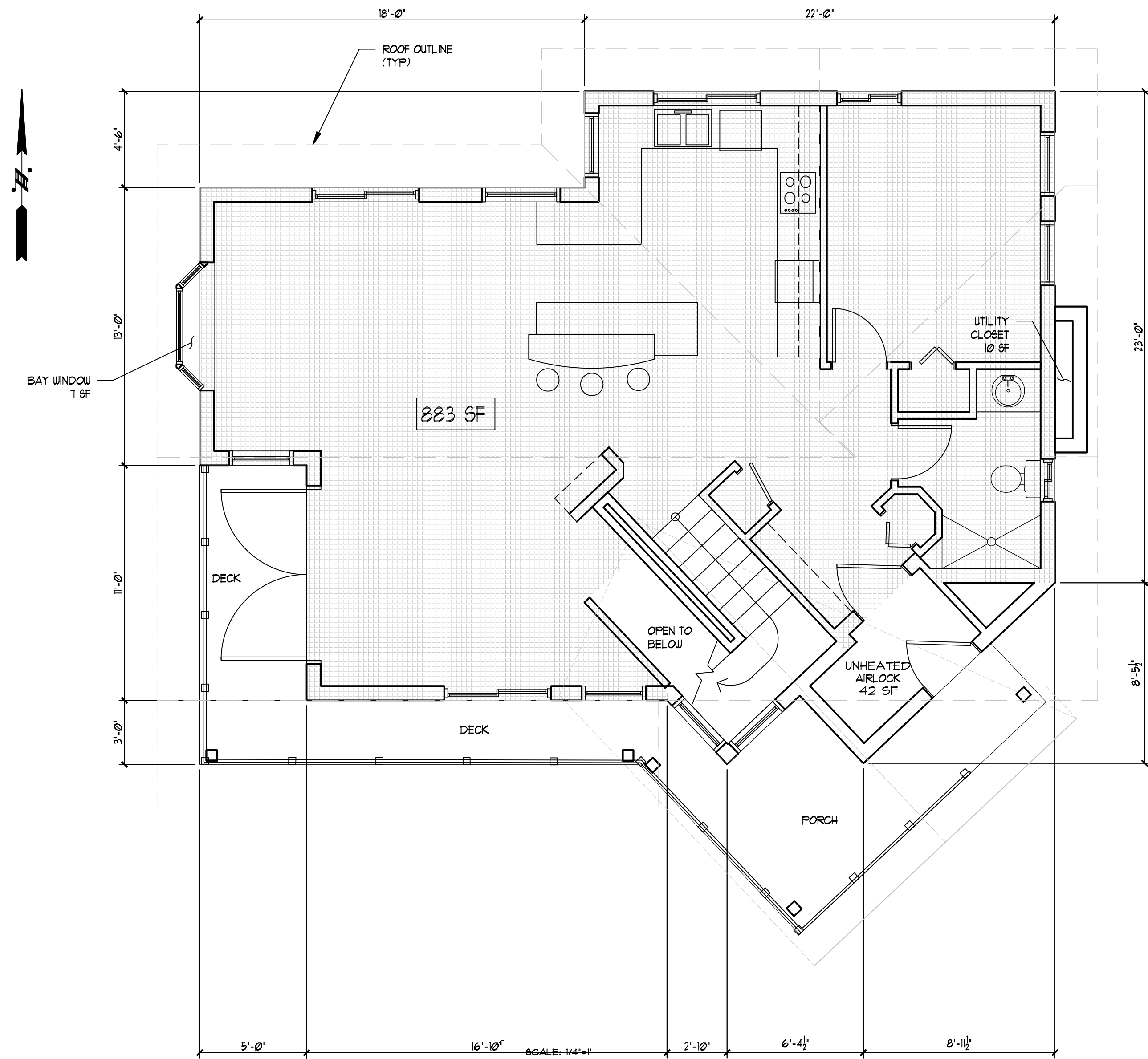
2 First Floor 06 SCALE: 1/4"=1' 883 SF (HEATED)
